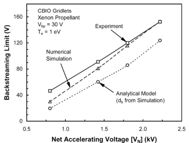
Fig. 13 Comparison between electron backstreaming measurements and simulation results.
